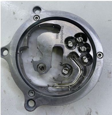
Figure 3. Titanium disc after CAD/CAM milling showing the frameworks still attached to the sprues after completion milling process.
